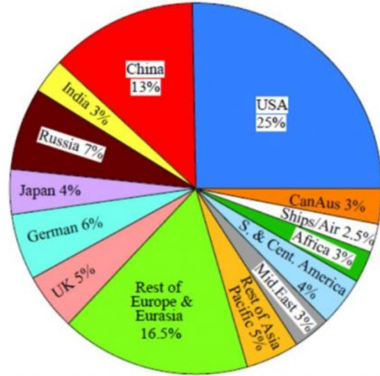
(b) 1751–2016 Cumulative Emissions
