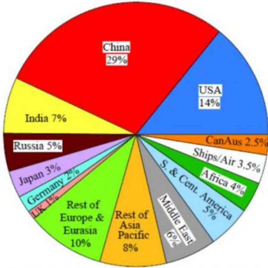
(a) 2016 Annual Emissions
